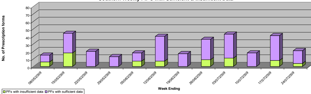
Southern Weekly P.F.'s with Sufficient & Insufficient Data
