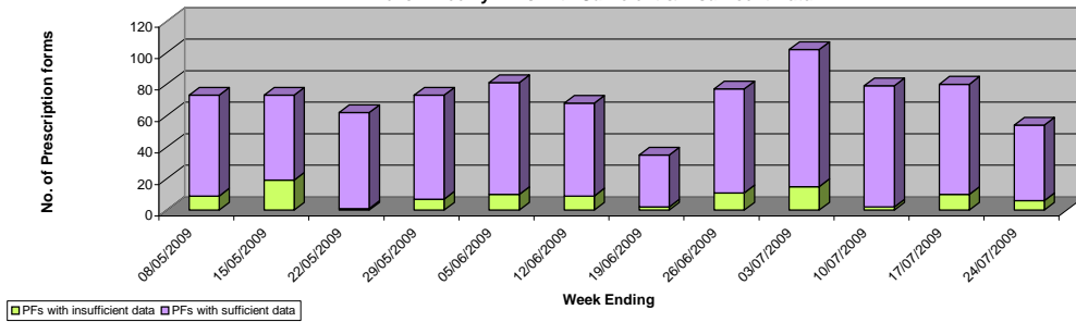
Devon Weekly P.F.'s with Sufficient & Insufficient Data
