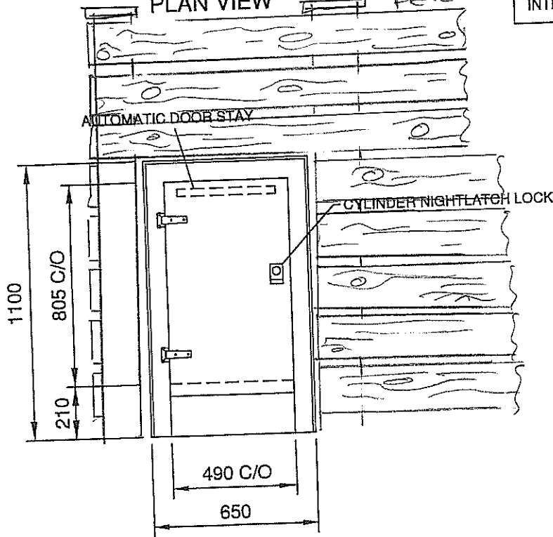
VIEW ON WALL 1
